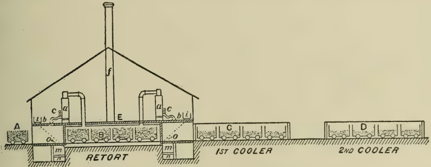
FIG. 76.—Modern Wood Distilling Plant.
